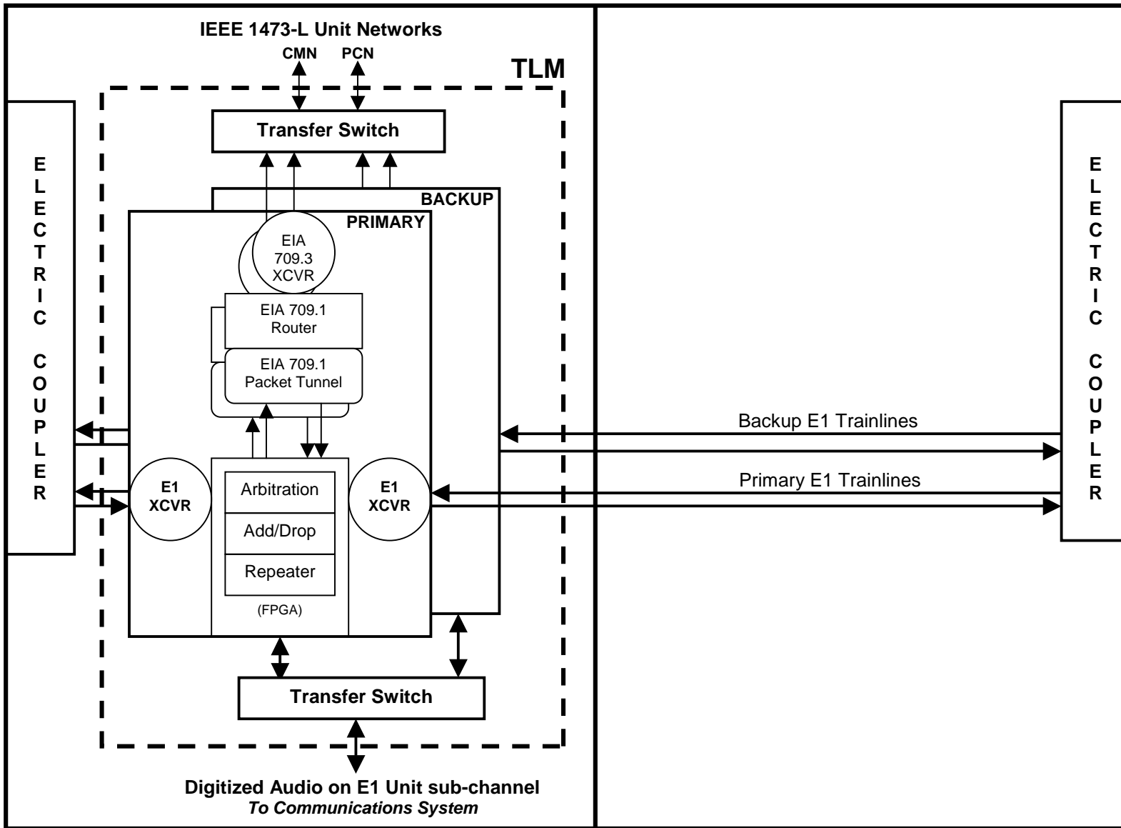
Redundant Add/Drop Trainline Multiplexer (TLM), IEEE 1473-L Networks and E1 Channels Conceptual Block Diagram
